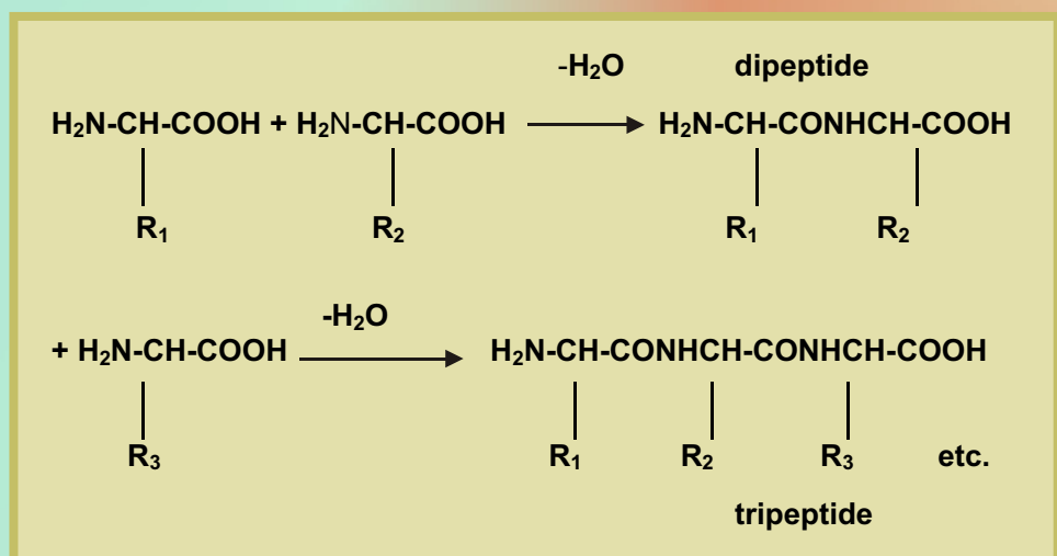
Figure 2: Formation of a polypeptide by reaction of amino acids. (R 1 , R 2 and R 3 may be the same or different side groups).
